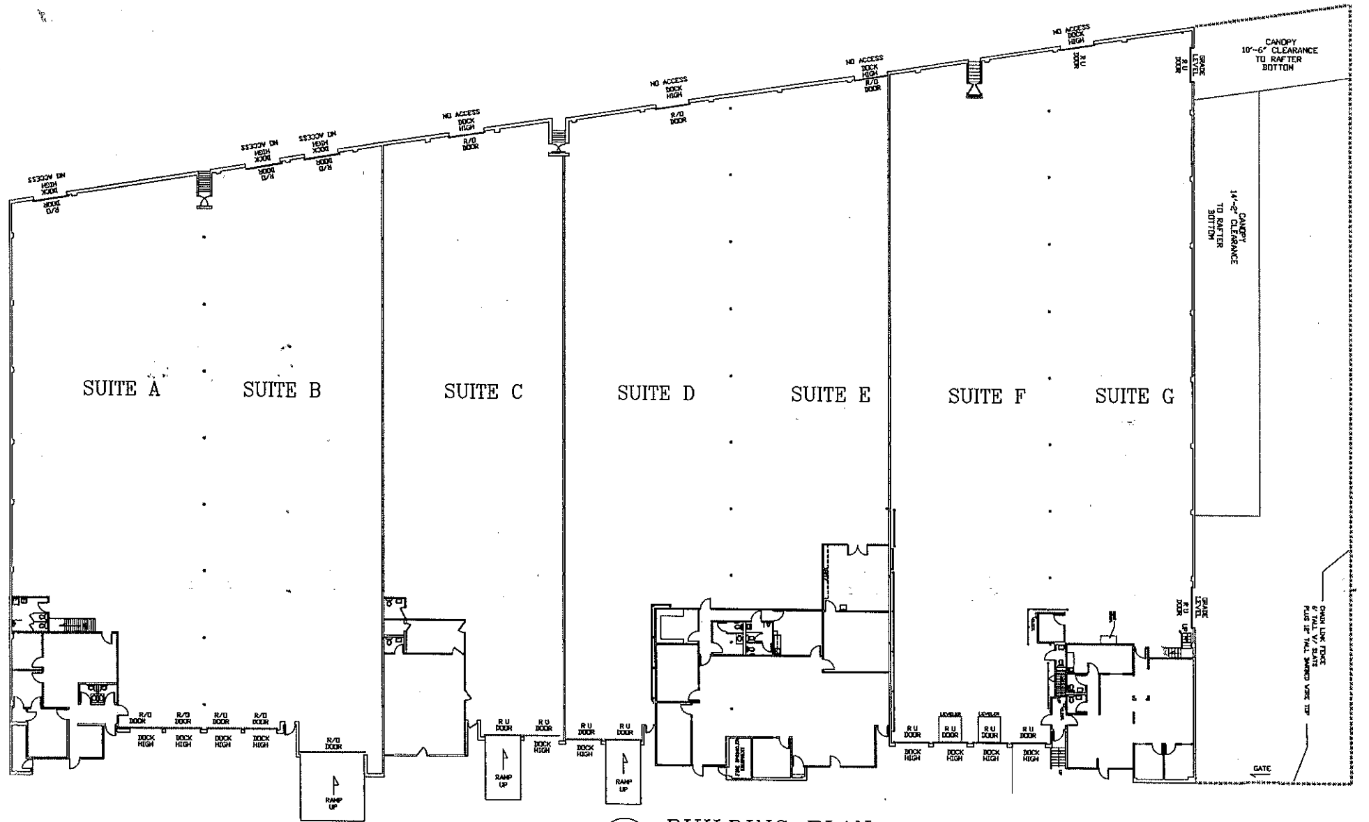
1 BUILDING PLAN 1 BUILDING #2 6870 N. FATHOM ST.
